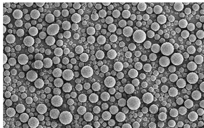
Bead polymers
