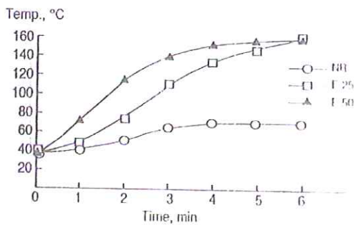
Figure 1 : Microwave energy absorption by Epoxyrenes
