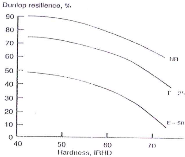
Figure 4 : Relilience of natural rubber and Epoxyprrens.
