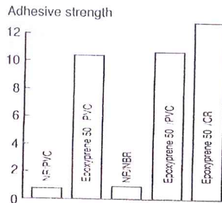
Figure 6 : Cured adhesion of Epoxyprrene
