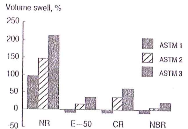
Figure 3 : Oil resistance of some selected polymers.
